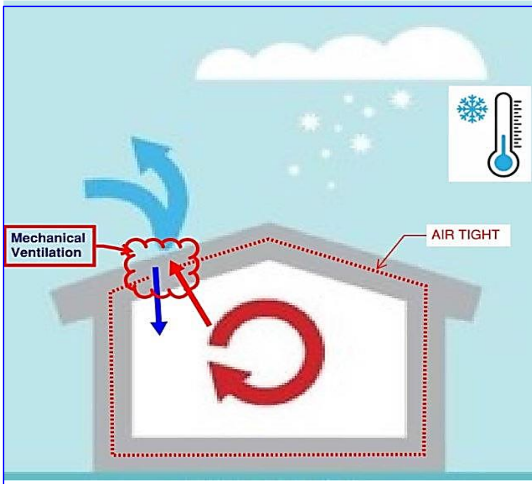
House with mechanical ventilation operating in cold snowy weather (windows closed)
