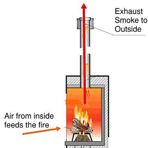
Open combustion where the fire consumes air in the house and smoke rising up the chimney
