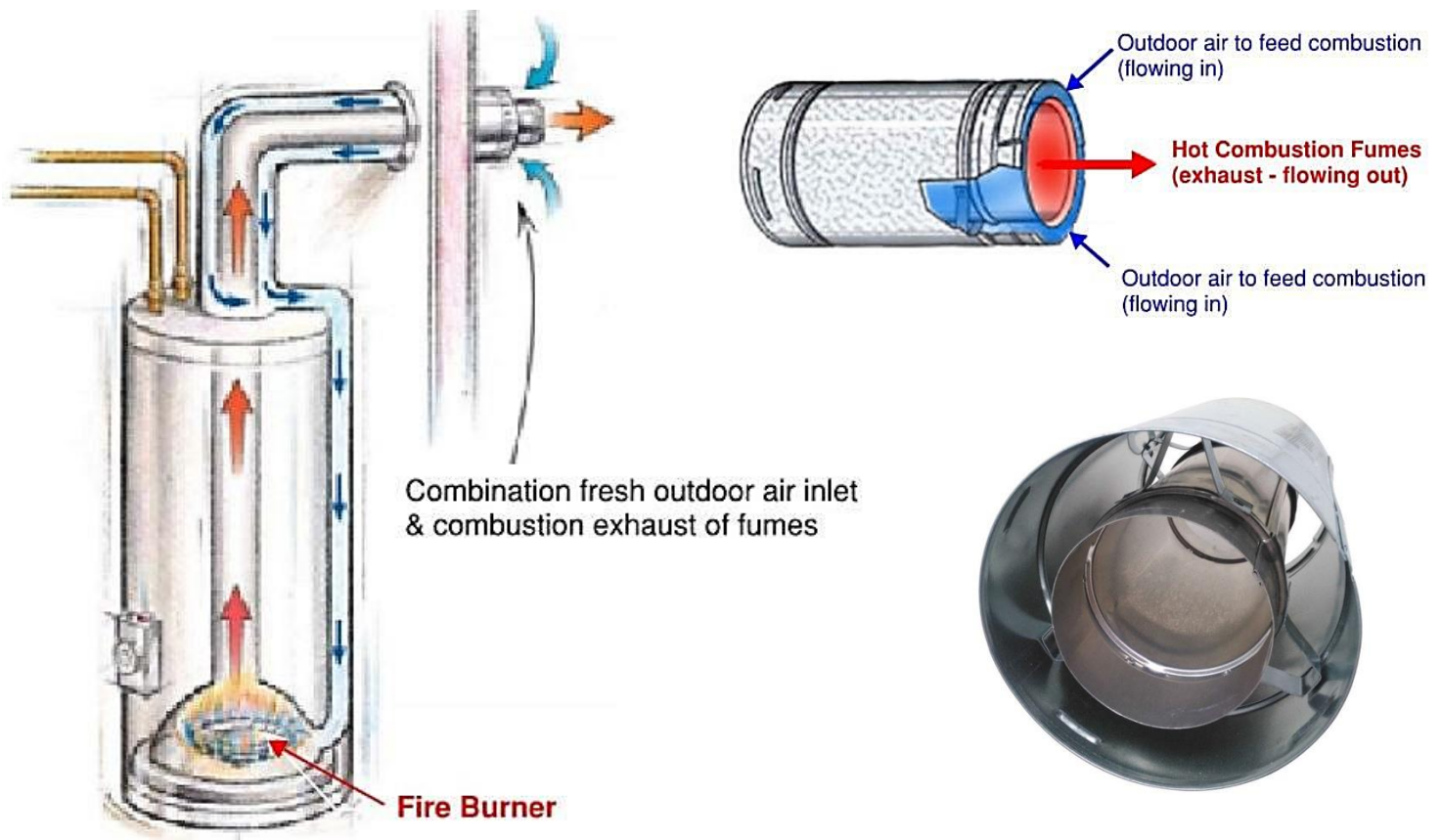
A fuel-burning hot-water tank direct-vented with a combined air-supply/exhaust vent (co-axial)
