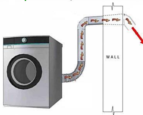
A laundry dryer exhausting directly through a wall to the outside
