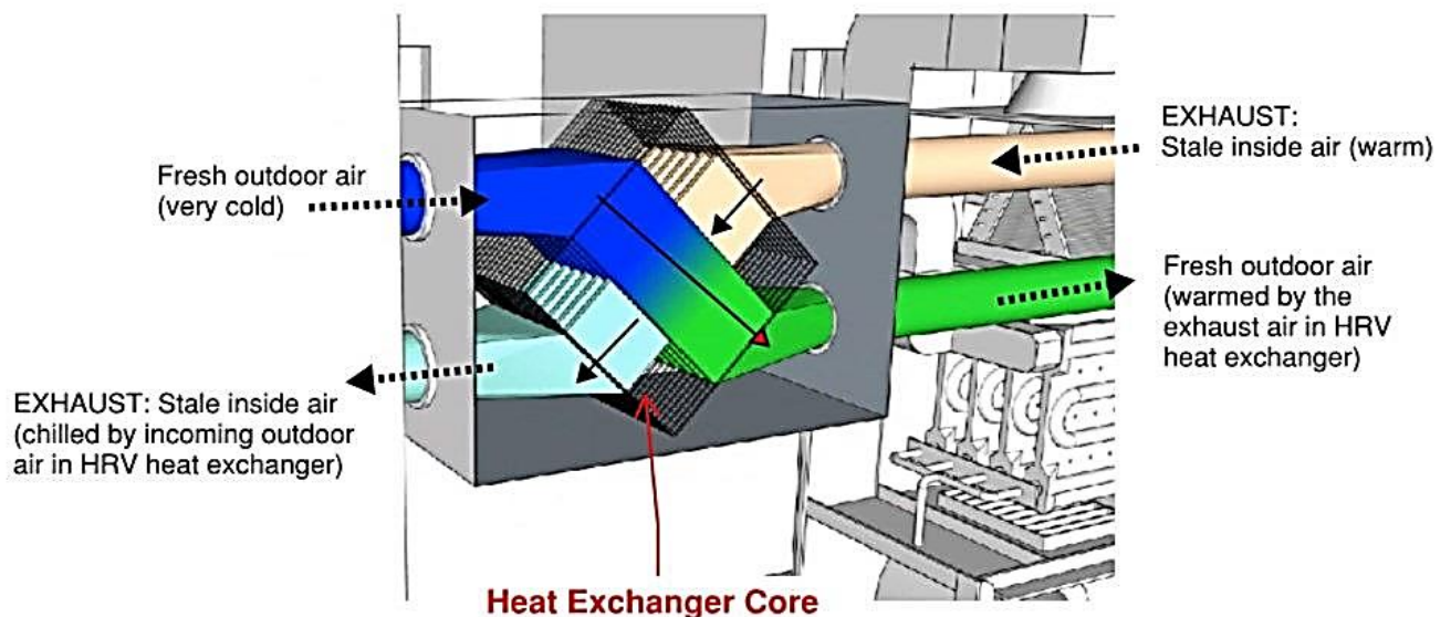
Exhaust air and incoming fresh outdoor air flow through a typical HRV or ERV
