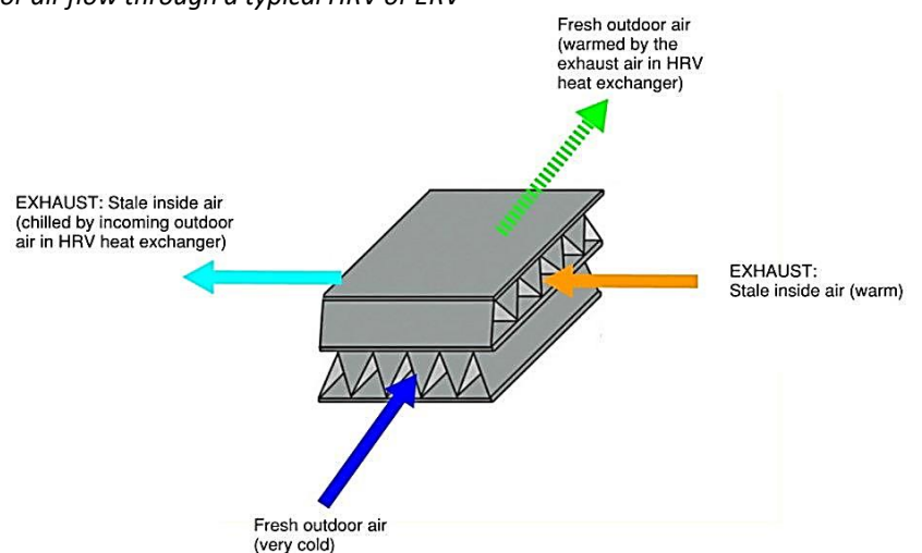
Typical offset channeled plates in the heat-exchanger core
