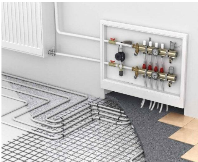
Hydronic radiant-heat flooring
