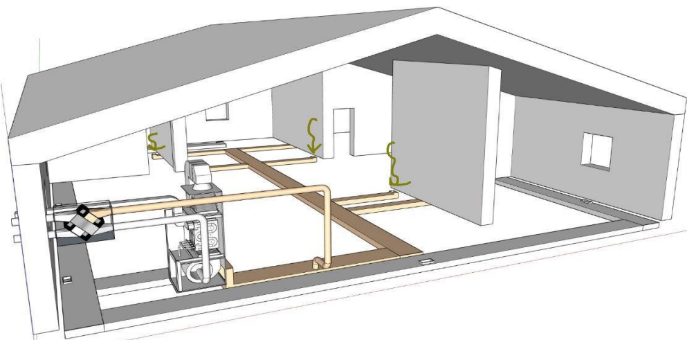
Return air-ducting in the middle of the house, away from exterior walls with vents at the base of interior partition walls
