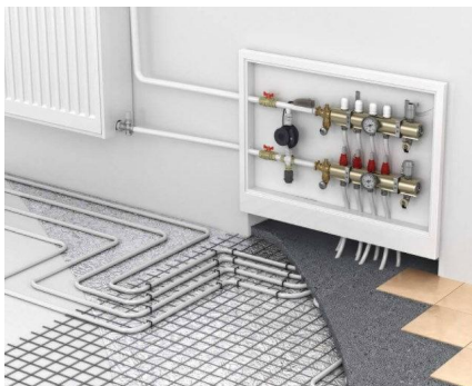
Hydronic radiant-heat flooring
