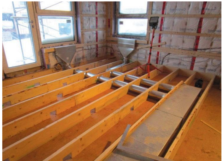
Air-distribution ducting installed in a floor service cavity
