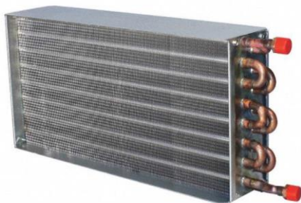
A hydronic heater designed to heat air in duct
