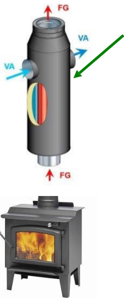
A typical wood stove
