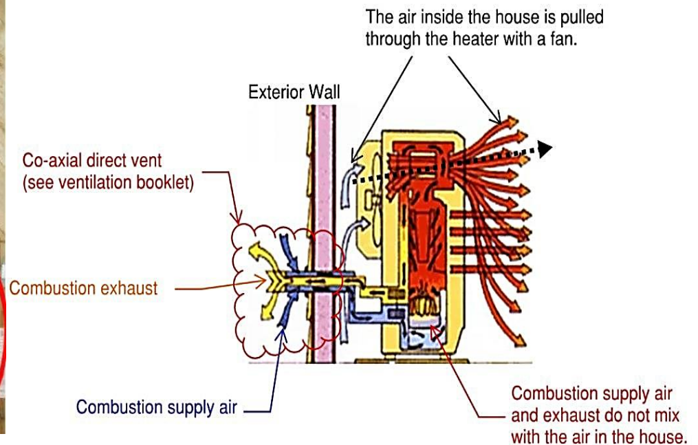
How the oil-burning unit heater works and needs its combustion gases (smoke) to exhaust through an exterior wall
